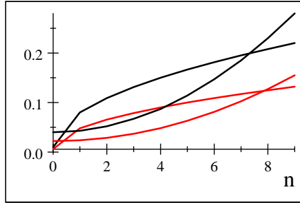
Figure 1: \phi and \alpha^w functions
